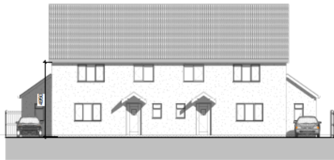
Front Elevation 1 : 100
